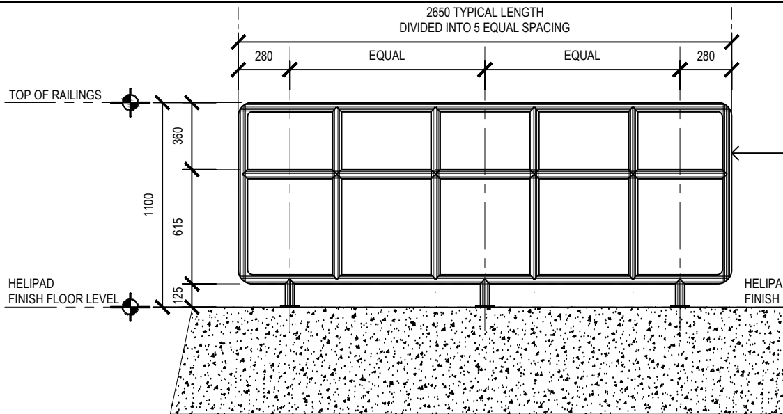
HELIPAD COLLAPSIBLE RAILINGS ELEVATION VIEW SCALE 1:20
