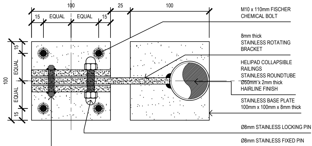
HELIPAD COLLAPSIBLE RAILINGS ROTATING PIN ASSEMBLY SCALE 1:2
